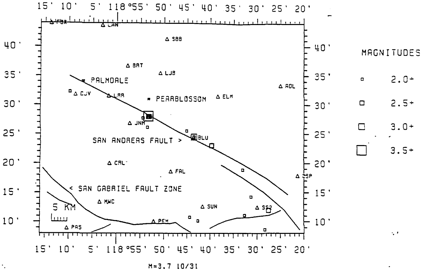
FIGURE 9: EARTHQUAKES ALONG SAN ANDREAS FAULT, JUL. - DEC. 1985
