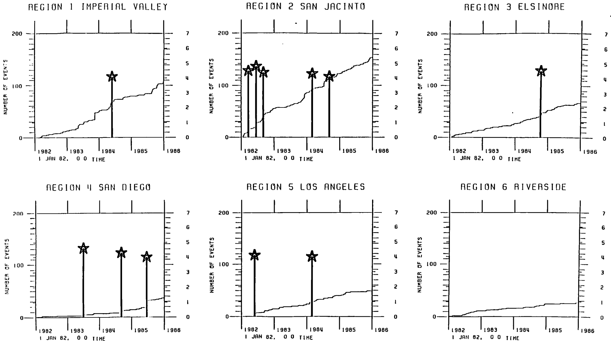
Figure 4: The cumulative number of earthquakes that occurred in regions 1-6 shown in figure 3 over the 48-month period ending December 31, 1985. All events of M = 2.5 or greater are included. The starred vertical lines denote earthquakes of M = 4.0 or greater (magnitude scales at right). Note that some regions extend beyond the area of complete station coverage.
