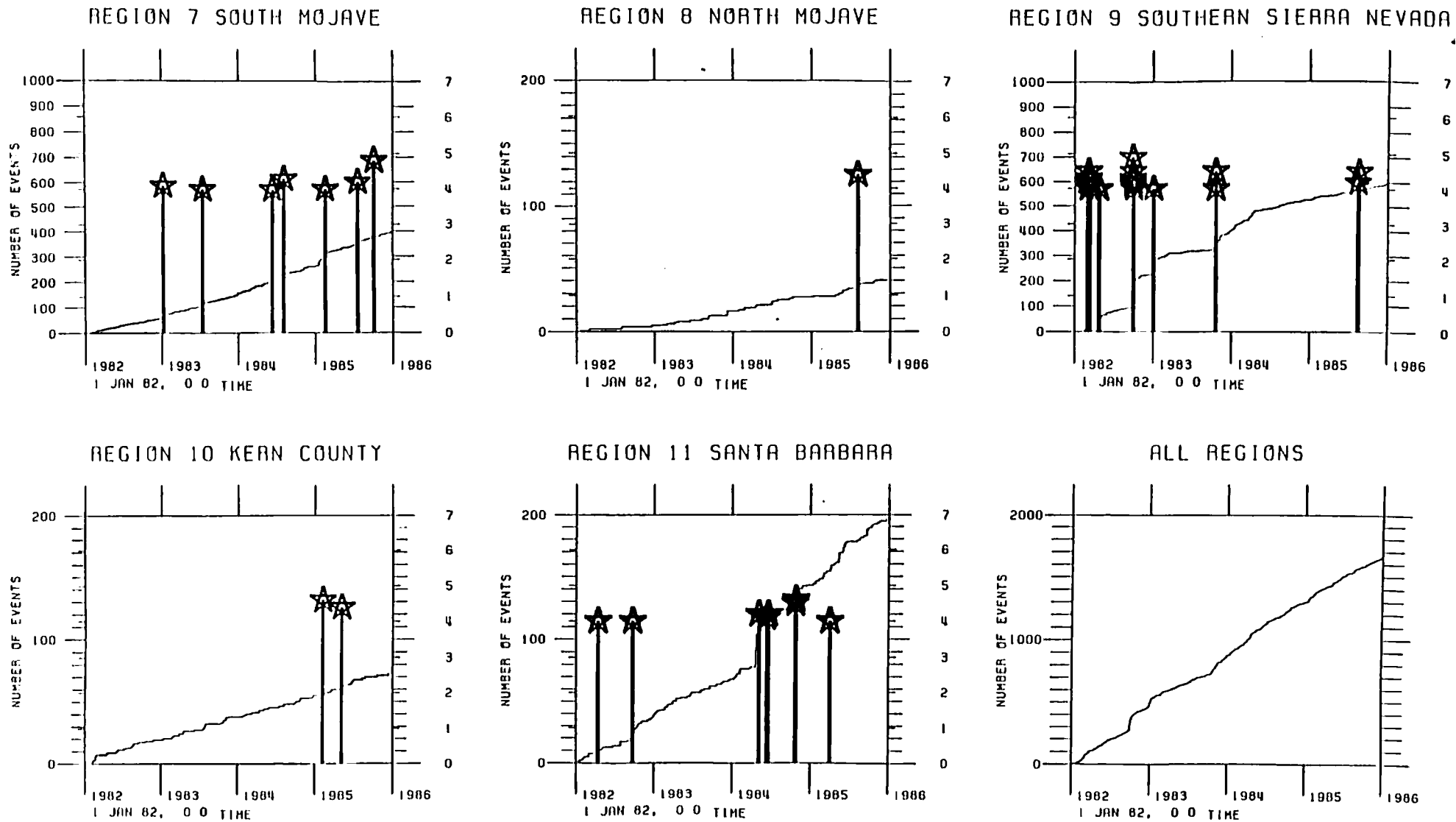
Figure 4: The cumulative number of earthquakes that occurred in regions 7-11 shown in Figure 3 over the 48-month period ending December 31, 1985. All events of M = 2.5 or greater are included. The twelfth plot displays the cumulative data from all 11 regions. The starred vertical lines denote earthquakes of M = 4.0 and greater (magnitude scales at right). Note that regions 7 and 9 have a different count scale than others, and that some regions extend beyond the area of complete stations coverage.
