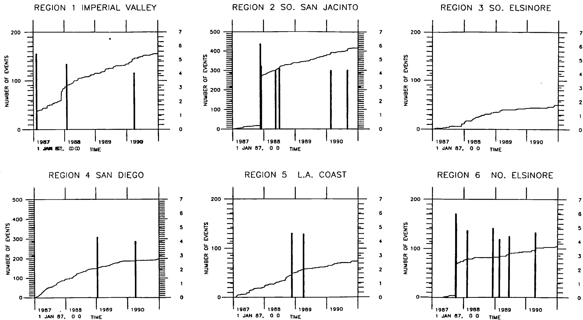
Figure 8a. Cumulative number of events ( M_L \geq 2.5 ) in sub-regions 1 through 6 over the four year period ending December 1990. The boundaries of the sub-regions are shown in Figure 7. Vertical bars represent time and magnitude (scale on right) of large events ( M_L \geq 4.0 ). Note that the vertical scales of the plots may not be the same.
