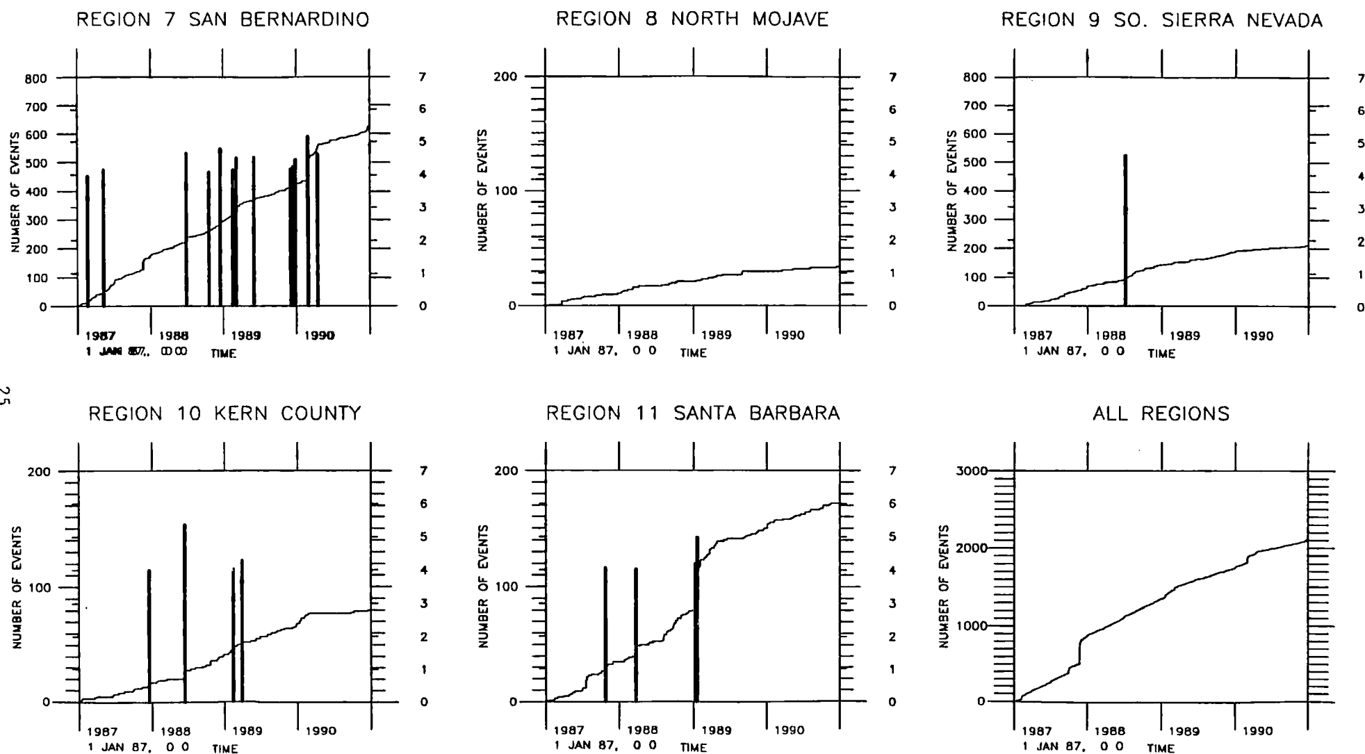
Figure 8b. Cumulative number of events ( M_L \geq 2.5 ) in sub-regions 7 through 11 and for all sub-regions over the four year period ending December 1990. The boundaries of the sub-regions are shown in Figure 7. Vertical bars represent time and magnitude (scale on right) of large events ( M_L \geq 4.0 ). Note that the vertical scales of the plots may not be the same.
